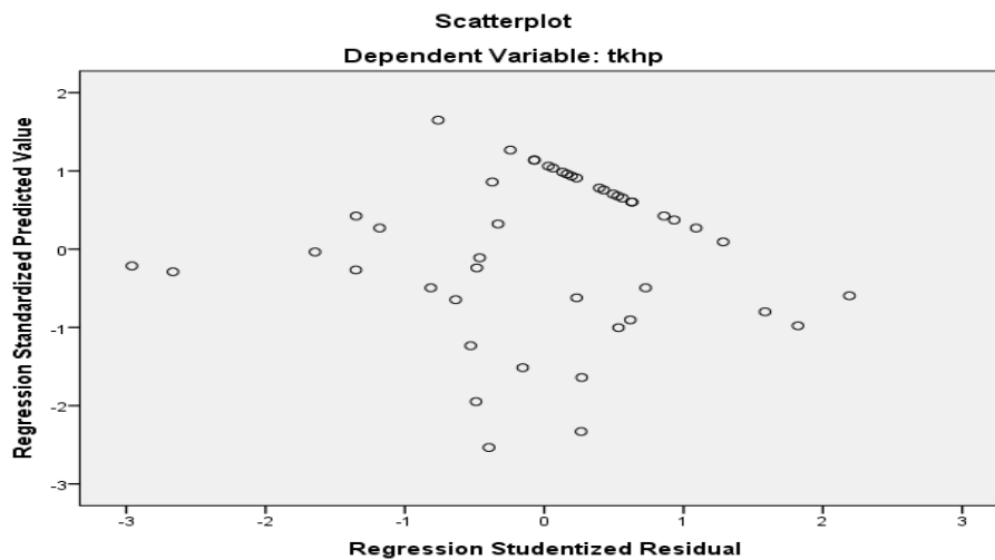
Gambar 1. Scatterplot
