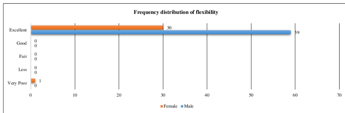
Figure 2. Frequency Distribution Diagram of Flexibility
