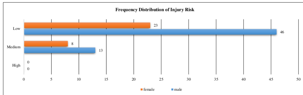
Figure 1. Frequency Distribution Diagram of Injury Risk
