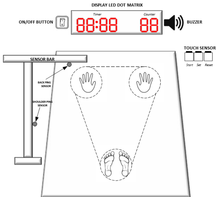
Figure 1. PUC Design
