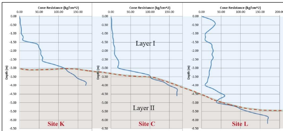
Fig. 6. Soil profile interpretation from CPT data of site K, C, L
