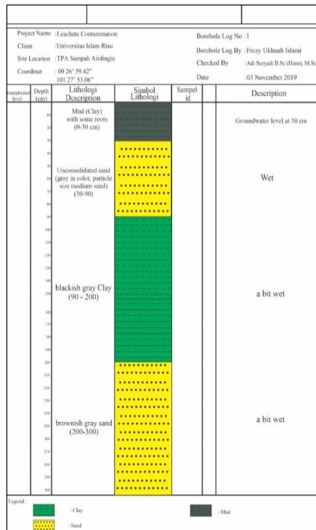
Figure 6. Hand Auger result that shown geological profile of subsurface at study area.
