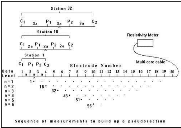
Fig 2. Equipment set up to acquisition resistivity data (Loke and Barker, 1995).
