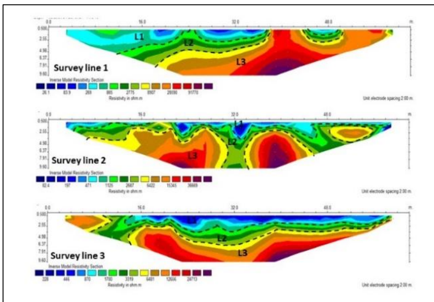
Fig 5. Result of resistivity survey from survey line 1, 2 and 3 that shown there are 3 layers named as L1, L2 and L3.
