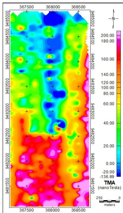
Fig 4. Contour map of TMA.
