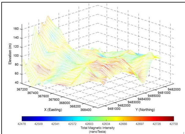
Fig 2. 3D distribution of TMI in the Tahi Ite village geothermal manifestation area.
