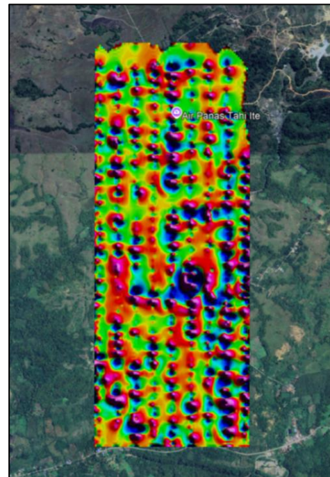
Fig 11. Overlay of SVD contour map on the Google Earth Pro imagery of the study area.
