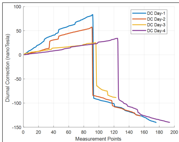
Fig 5. Diurnal correction (DC) values for each measurement point during the four day measurement period.
