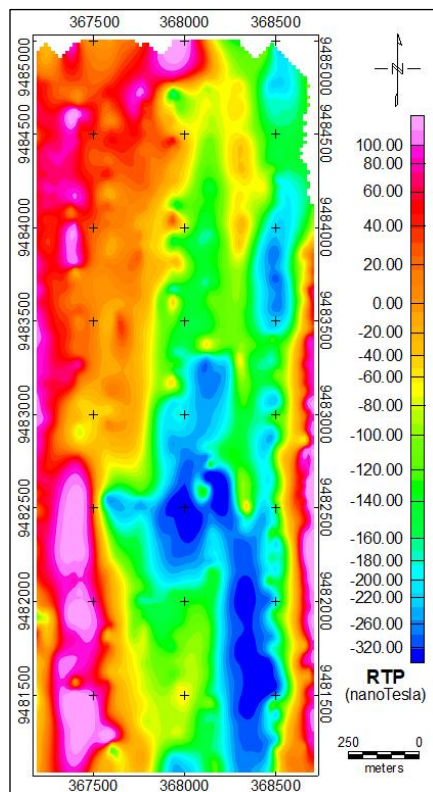
Fig 7. Contour map of RTP result on LMA in the Tahi Ite Village geothermal area.
