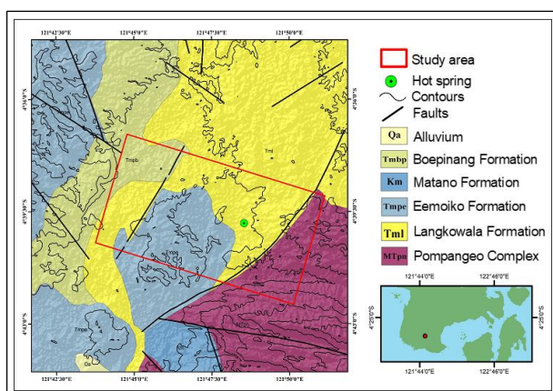
Fig 1. Distribution map of rock formations in Tahi Ite Village (modified from Simandjuntak et al. (1993)).
