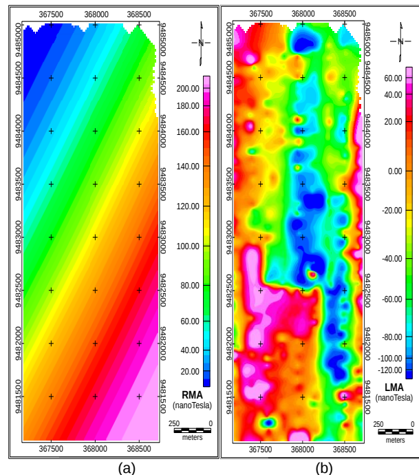
Fig 6. Contour map of magnetic anomalies in the Tahi Ite geothermal area: (a) RMA and (b) LMA.
