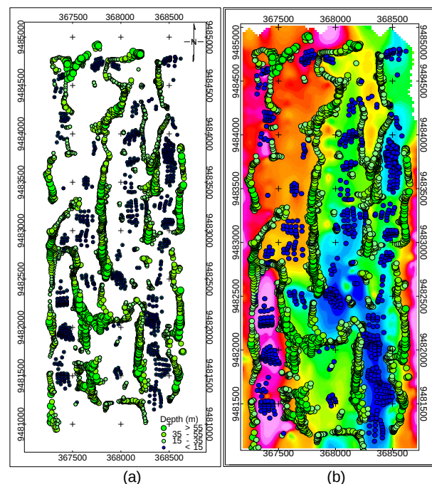
Fig 8. (a) Euler Deconvolution results for N=0 Structural Index, and (b) overlay of the Euler solutions on LMA contour map.
