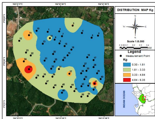
Fig. 6 Distribution Map of Seismic Vulnerability Index ( K_g )
