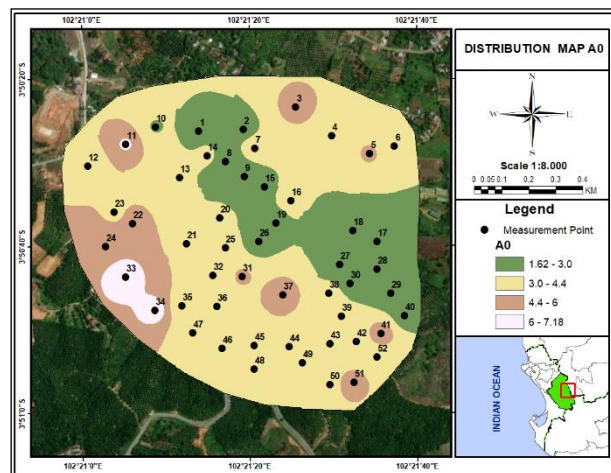
Fig. 5 Distribution Map of Amplification ( A_0 )
