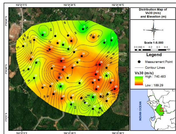
Fig. 7 Distribution Map of V_{s30} (m/s) and Elevation (m)
