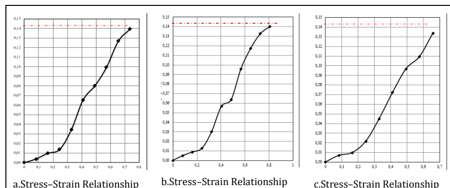
Fig 2. Graph of Normal Sample 1 (a), Normal Sample 2 (b), and Normal Sample 3 (c) (Source: processed data, 2025)
