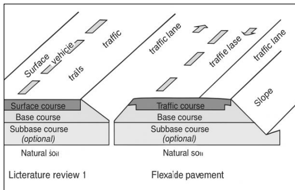
Fig 1. Cross-Section of Conventional and Flexaide Pavement Structures (Yunus, 2024).
