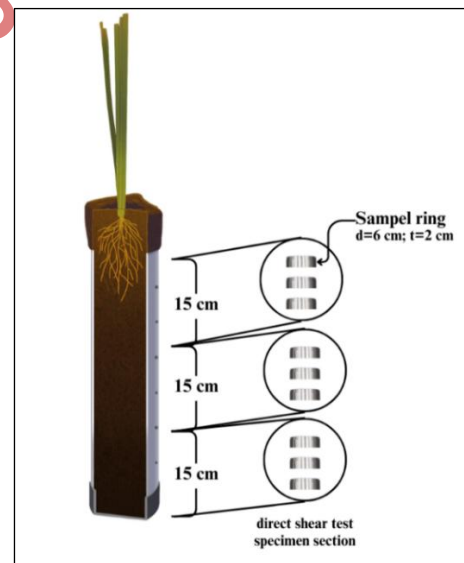
Fig. 4 Schematic of shear strength test
