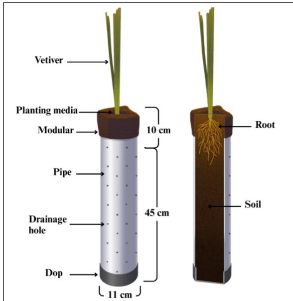
Fig. 3 Schematic of vetiver planting with modular on pipes
