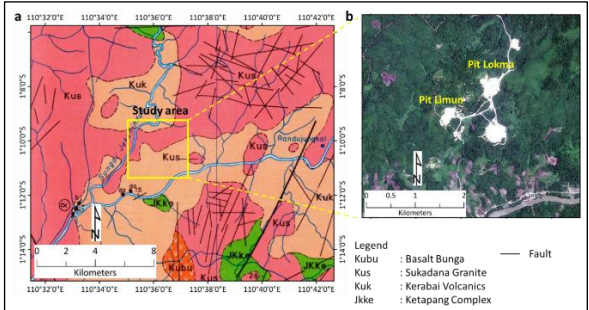
Fig. 1. (a) Regional geological map of the study area showing the distribution of lithologies, including the Sukadana Granite (Kus) and surrounding volcanic units, with the study area outlined in yellow (modified from Rustandi and De Keyser, 1993). (b) Situational map of Pit Lokma and Pit Limun within the study area, overlaid on true-color PlanetScope Basemap (@PlanetScope) satellite imagery acquired in September 2024.
