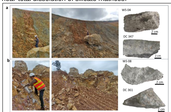
Fig. 2. Field exposures and representative hand specimens from (a) Pit Limun and (b) Pit Lokma. (a) Pit Limun: field exposures showing altered andesitic wall rocks with limonite staining and quartz–pyrite veinlets; WS 04: intensely sericitized andesite with quartz flooding and pyrite disseminations; DC 347: dark grey hydrothermal breccia with sericite–quartz–pyrite alteration and sulfide mineral indications. (b) Pit Lokma: field exposures showing intensely altered and brecciated zone with reddish-brown iron oxide-stained matrix; WS 08: pale grey, leached clay-rich rock; DC
