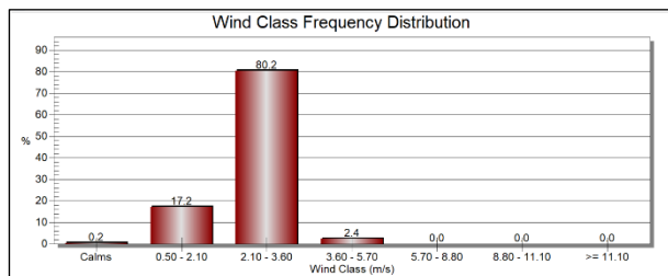
Fig. 3 Muko Muko Wind Class Frequency Distribution of Wet Season
