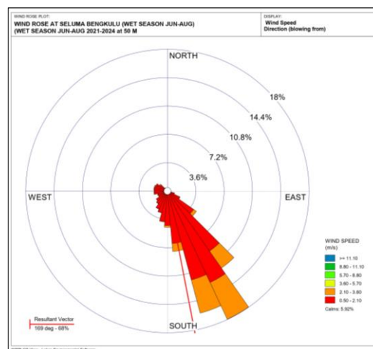
Fig 9. Seluma Wind rose Diagram in June – August in Year of 2021 – 2024
