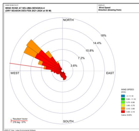
Fig 10. Seluma Wind rose Diagram in December – February in Year of 2021 – 2024
