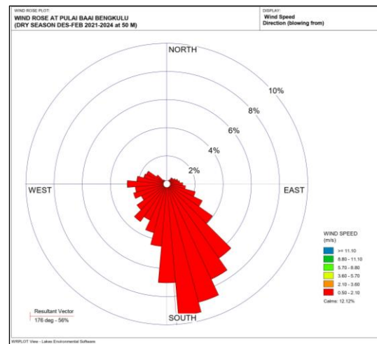
Fig 5. Baai Island Wind rose Diagram in June – August in Year of 2021 – 2024
