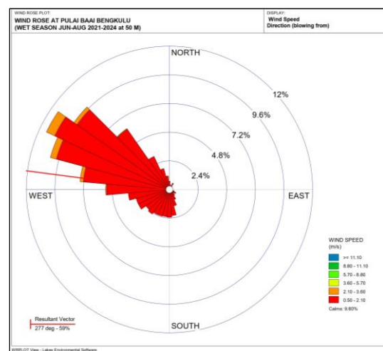
Fig 6. Baai Island Wind rose Diagram in December – February in Year of 2021 – 2024
