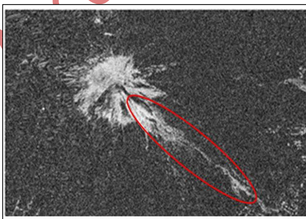
Fig 4. DEM Image Before Mount Semeru Eruption
