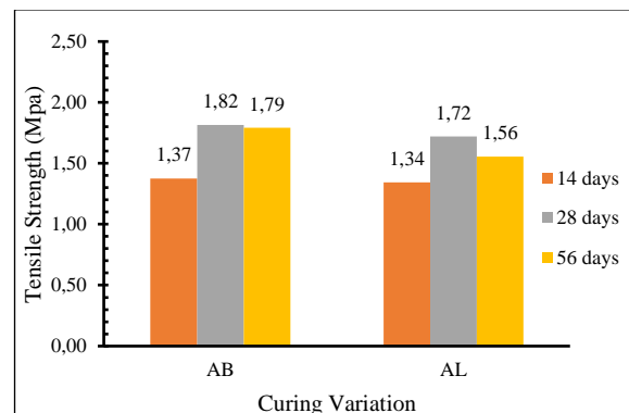
Fig. 7. Tensile Strength Result
