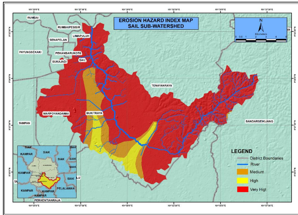
Fig 9. Erosion Hazard Index Map in the Sail Sub-Watershed
