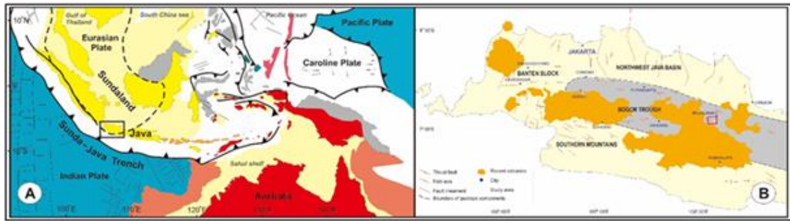
Fig. 1 (A) Tectonic frameworks of Indonesian region, represents the Sunda-Java Trench where the Australian plate subducts beneath Eurasian continent to the north. The Sundaland seated on the southern margin of this Eurasian continent (Hall, 1996). (B) Tectonic elements of West Java, E-W elongate of Bogor Trough in the center part through the east. Red rectangular indicated the study area in the center part of Bogor Trough. Modified mainly after Martodjojo (2003) and Satyana & Armandita (2004)
