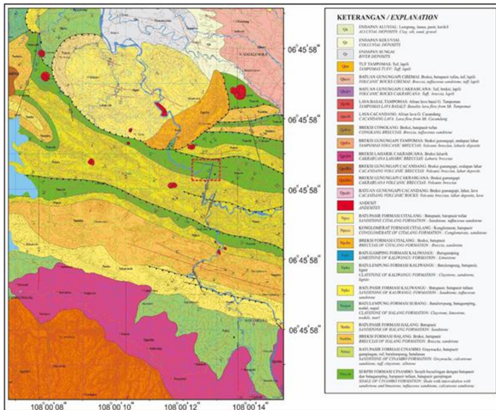
Fig. 2. Geological map of Majalengka Area (Isnaniawardhani et al., 2020), shows relatively E-W Neogene deposits distribution, following folds and thrust system in this region. Rectangular red dot is the study area, part of the oldest stratification of Cinambo Formation.
