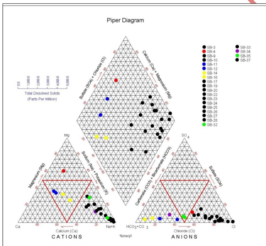
Fig 2. Result of Piper diagram analysis
