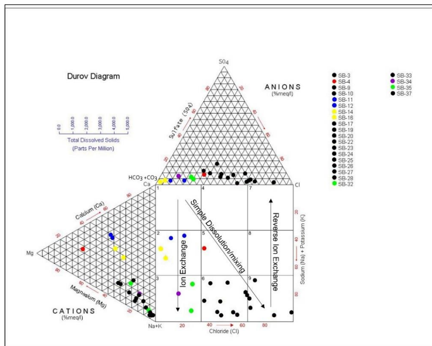
Fig 4. Durov diagram shows the interaction mechanism of ion
