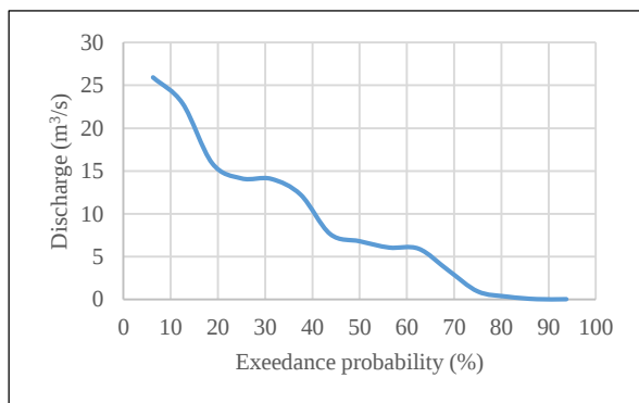
Fig 10. October duration curve
