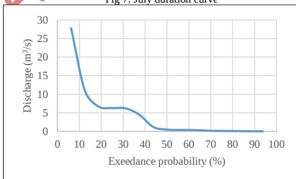
Fig 7. July duration curve
