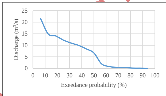
Fig 7. July duration curve
