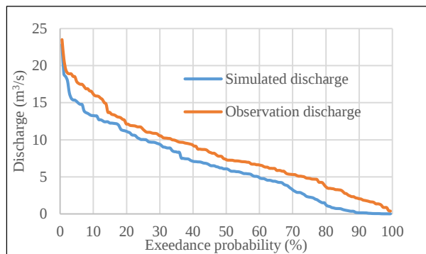
Fig 4. Duration curve calibration (Cimanuk-Bayongbong catchment area)
