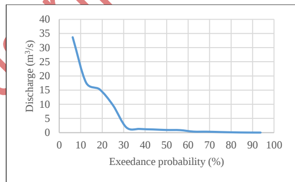
Fig 9. September duration curve
