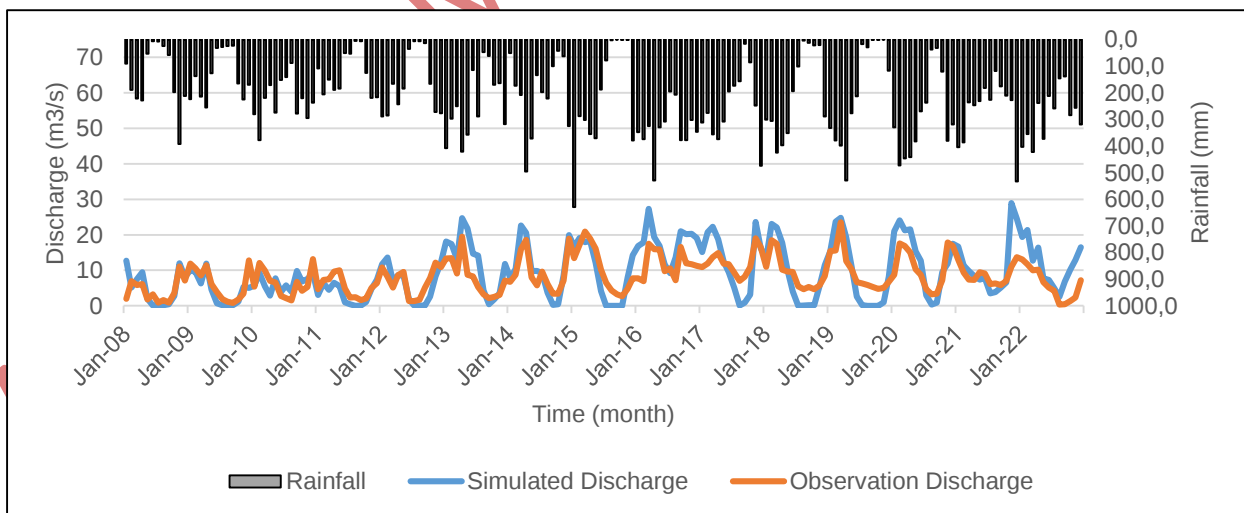
Fig 3. Time series calibration (Cimanuk-Bayongbong catchment area)
