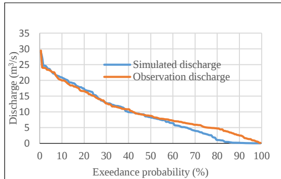
Fig 6. Duration curve calibration (Cimanuk-Bojongloa catchment area)
