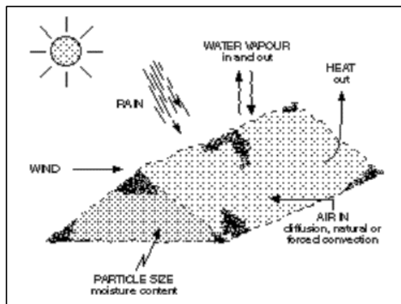
Fig. 1. Factors causing Self-Heating in the Stockpile Area (Carras et al., 1994)
