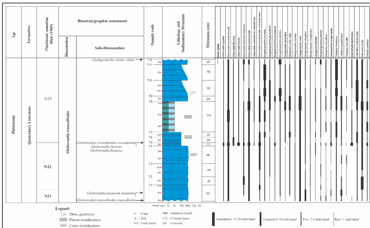
Fig 5. Biostratigraphic ranges of planktonic foraminifera taxa in Taeno Traverse, consisting of three biozonations, N21, N22, and N23, indicate Pleistocene age.
