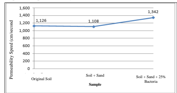
Fig 6. Graphic of 26°C water temperature permeability coefficient The results of Figure 6 on the graph, the permeability value with a mixture of sand and 25% bacteria and a water
