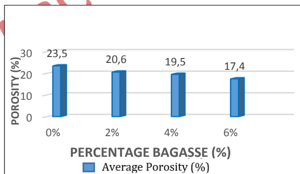
Fig 4. Comparison of Bagasse Addition Percentage with Porosity.
