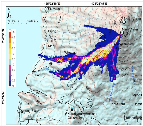
Fig 13 (a). Case 1 with 500 \times 10^3 m 3 and \mu 0.5
