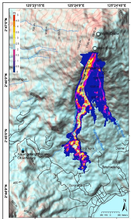
Fig 8 (f). Case 6 1500 \times 10^3 \text{ m}^3 with \mu 0.7
