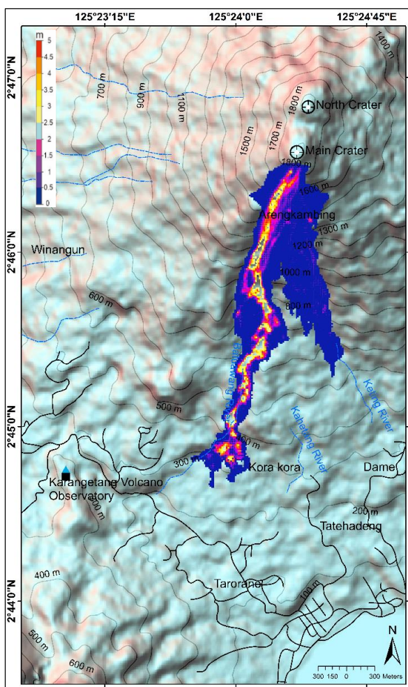
Fig 8 (a). Case 1 with 500 \times 10^3 m 3 and \mu 0.5
