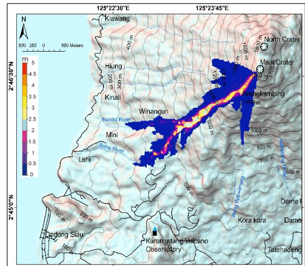
Fig 13 (b). Case 2 with 1000 \times 10^3 m 3 and \mu 0.5
