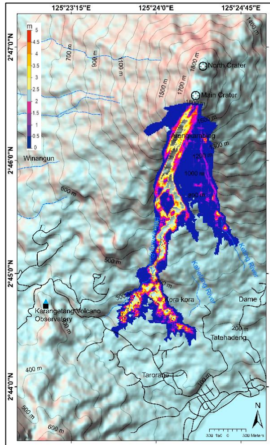
Fig 8 (e). Case 5 1500 \times 10^3 \text{ m}^3 with \mu 0.5
