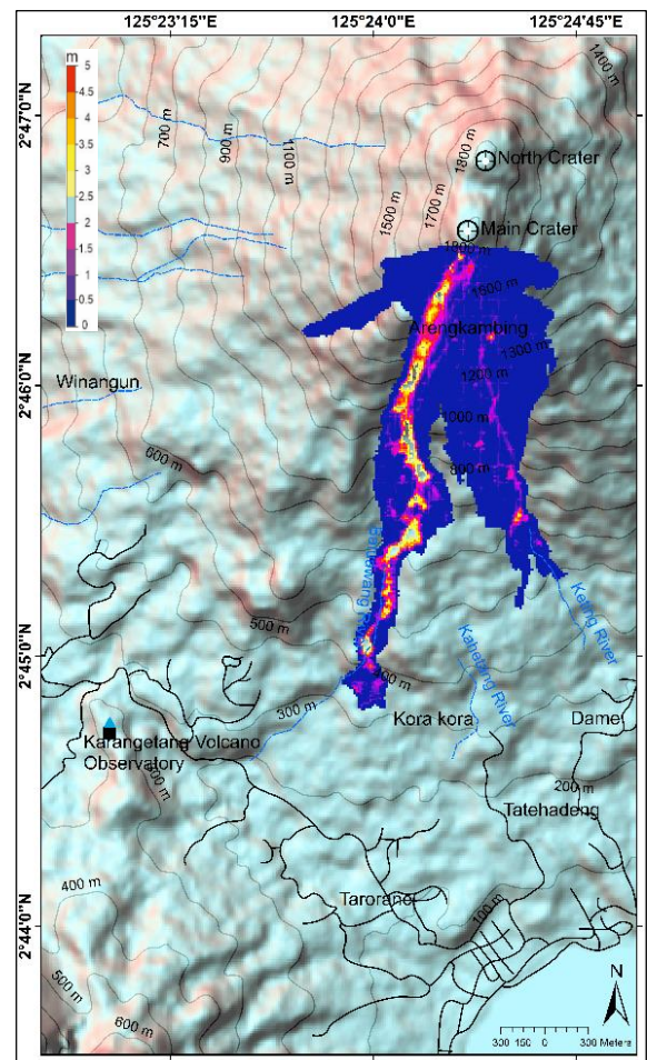
Fig 8 (b). Case 2 with 500 \times 10^3 m 3 and \mu 0.7
