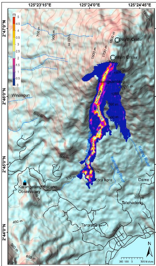
Fig 8 (d). Case 4 with 1000 \times 10^3 \text{ m}^3 and \mu 0.7
