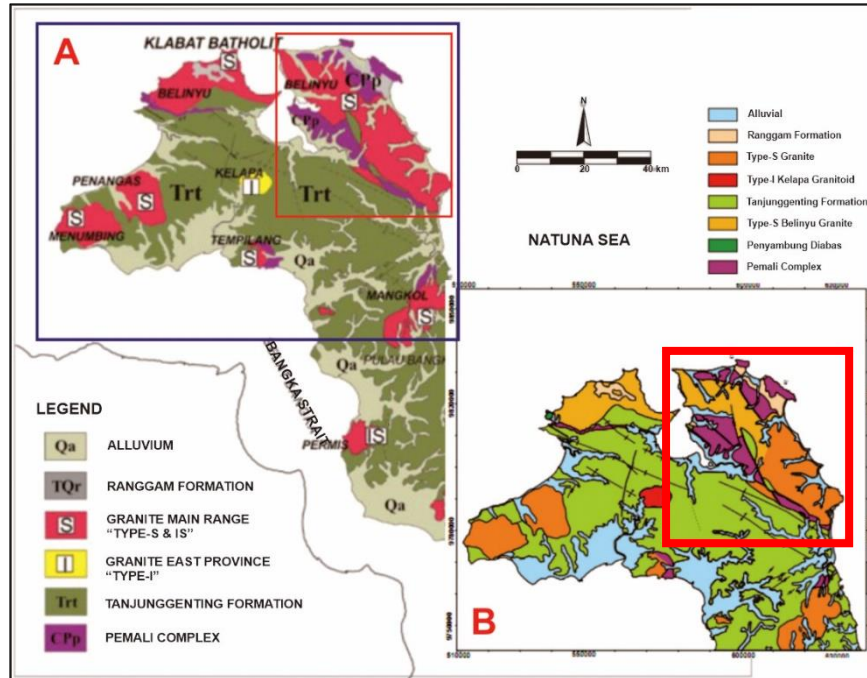
Fig. 2. (A) Geology map of Bangka with red square as a research area (Barber et al., 2005; Cobbing et al., 1986; Mangga and Djamal, 1994; Margono et al., 1995; Sugiono, 2014) (B) Map of granite type in northern Bangka Island.
