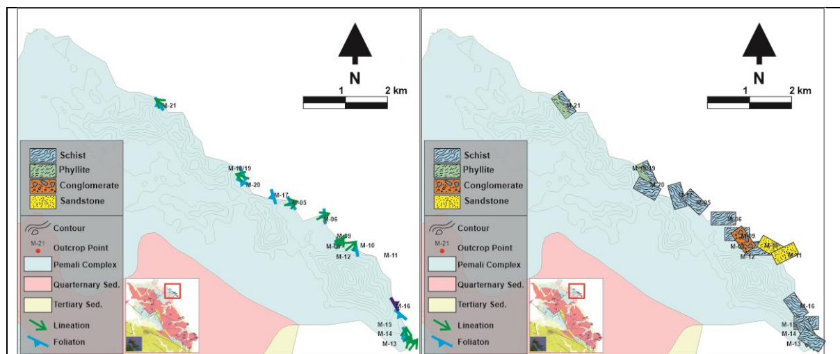
Fig. 4. Structural map with foliation and lineation (A) Outcrop distribution in the research area (B).
