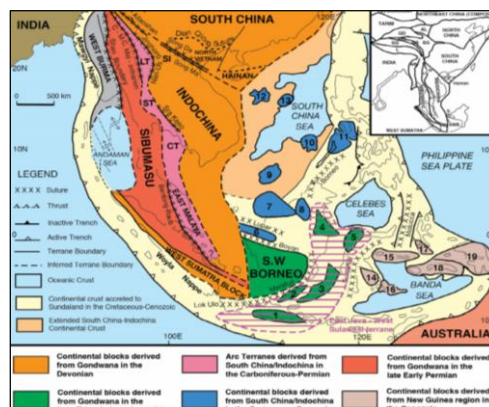
Fig. 1. Distribution of continental blocks, fragments, terranes, and principal sutures of Southeast Asia (Metcalf, 2013).
