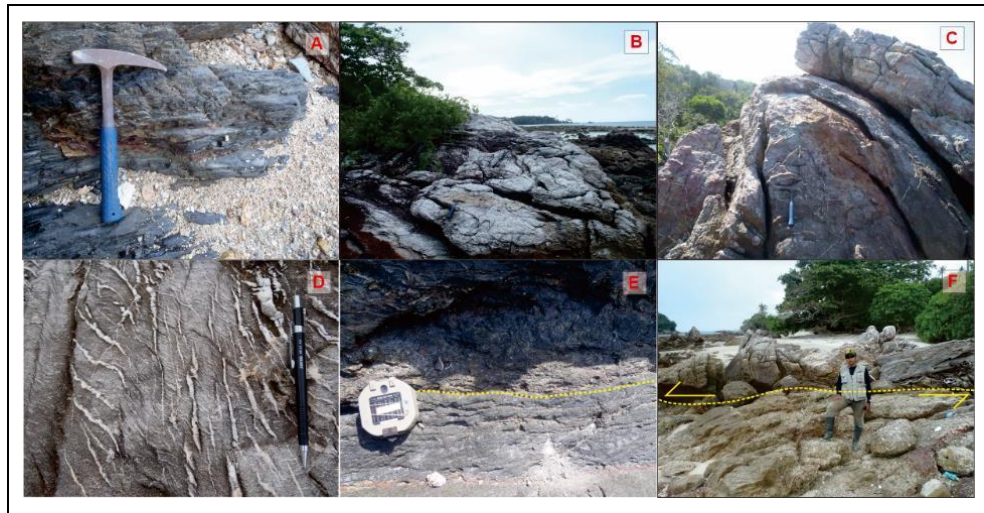
Fig. 5. Several macrostructures occurrences in field area (A) parallel foliation, (B) Foliation in schist, (C) Fold in crystalline rocks, (D) Enchelon vein and crenulation cleavage, (E) S-C fabric, (F) Strike-slip fault.
