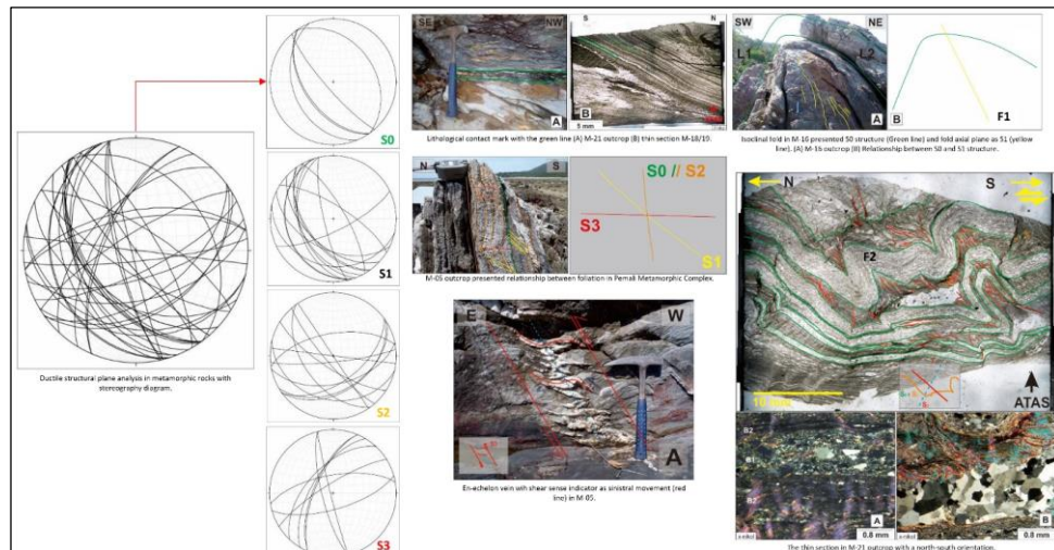
Fig. 6. Scheme of foliations list in the research area.
