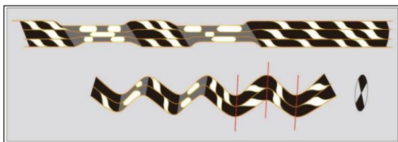
Fig. 8. Second deformation phase (D2) associated with fold (F2) and foliation S1 (yellow line), foliation S2 (orange line), and foliation S3 (red line) modified from (Schavemaker et al., 2012).
