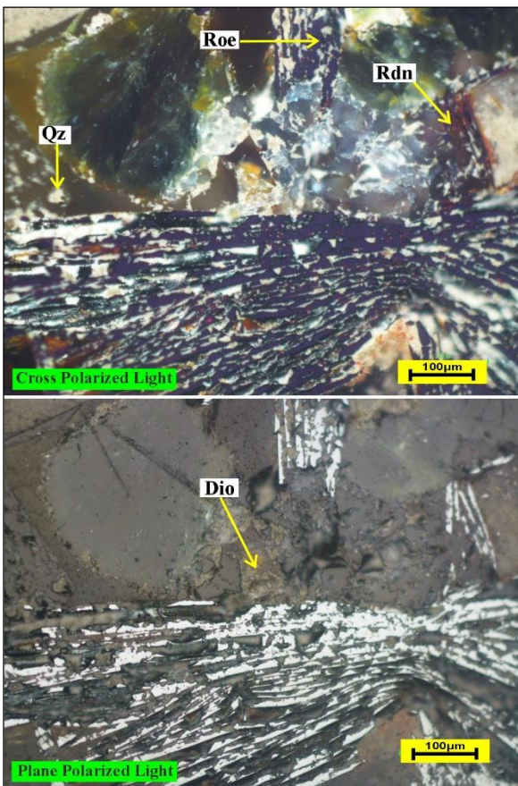
Fig. 9. Photomicrograph result of mineralogical analysis samples 1 (Rb=Roeblingite, Rhd= Rhodonite, Qz=Quartz, Dp=Diopside)
