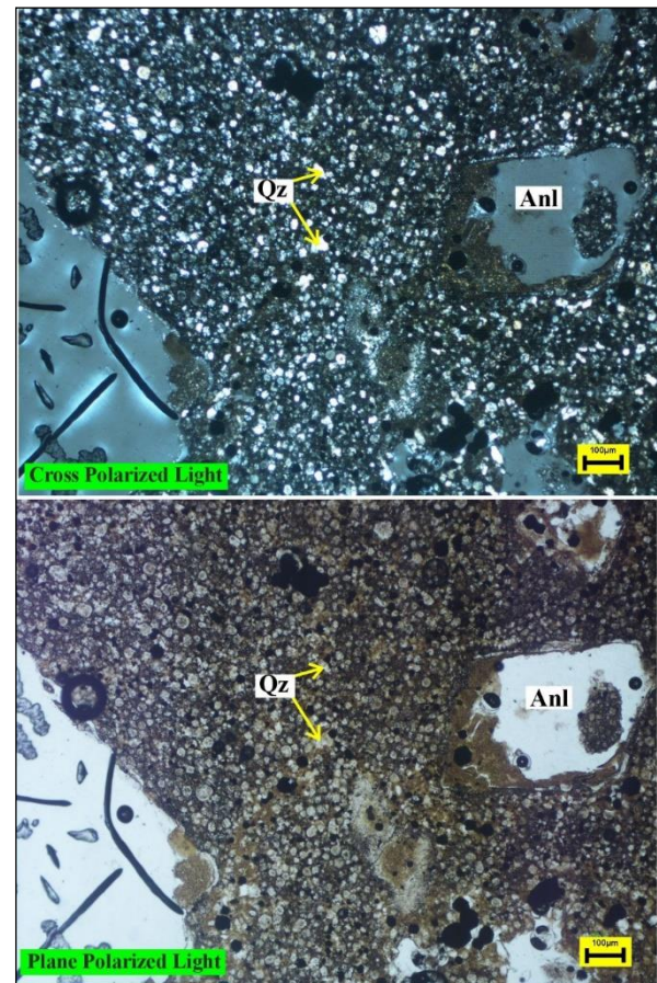
Fig. 11. Photomicrograph result of petrographic analysis samples 3 (Anc=Analcime, Qz=Quartz, Plg=Palygorskite)
