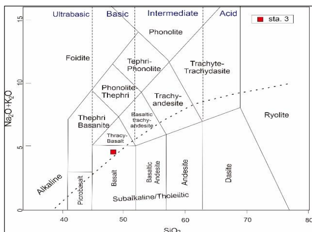
Fig. 12. Classification of rock types according to (Bas et al., 1986)
