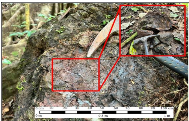
Fig. 3. Description of Station 1 manganese minerals
