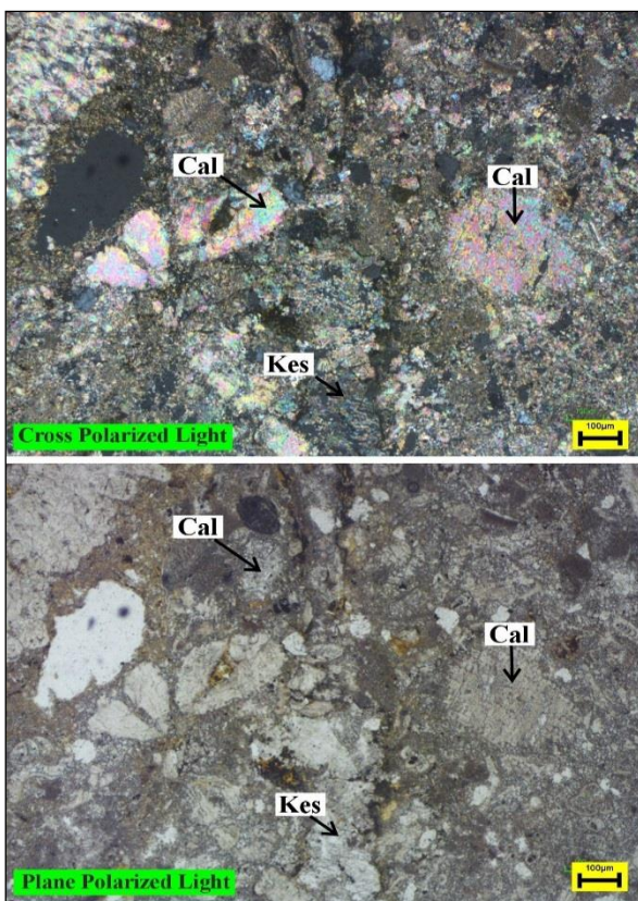
Fig. 10. Photomicrograph result from petrographic analysis samples 2 (Ks=Calcite, Krs= Krieselite)
