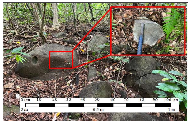
Fig. 5. Description of Station 3 Porphyry basalt
