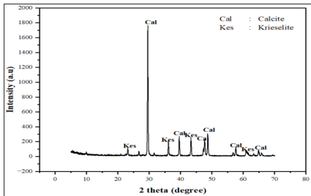
Fig. 7. Diffractogram result in XRD analysis station 2
