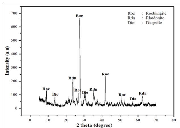
Fig. 8. Diffractogram result in XRD analysis station 3
