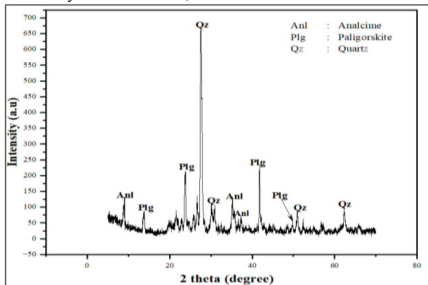
Fig. 6. Diffractogram result in XRD analysis station 1
