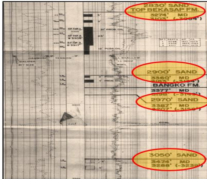
Gambar 7 Marked Log Sumur BA#147
