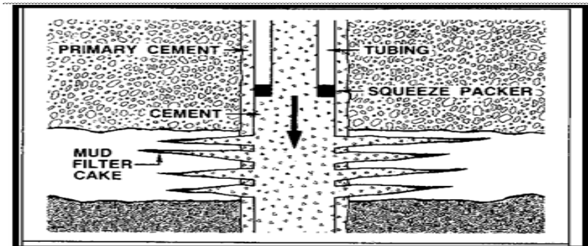
Gambar 6 Packer Squeeze (Nelson, 1990)
