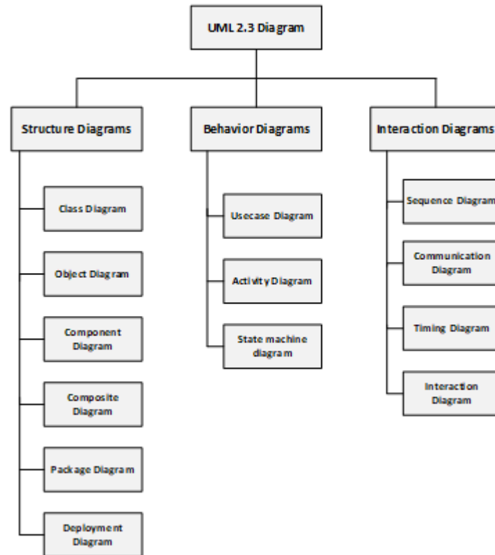
Gambar 2. Diagram UML
