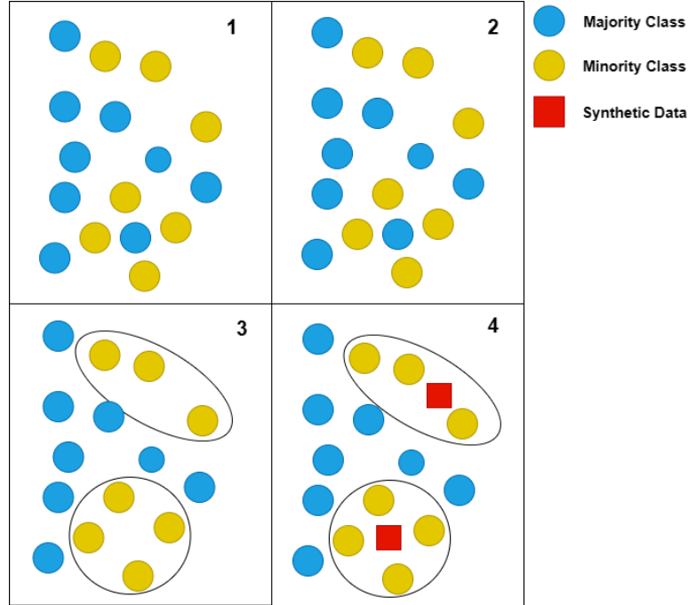
Figure 2. MWMOTE
